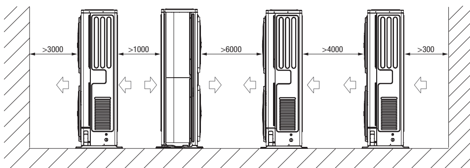
For parallel installation in a several row
