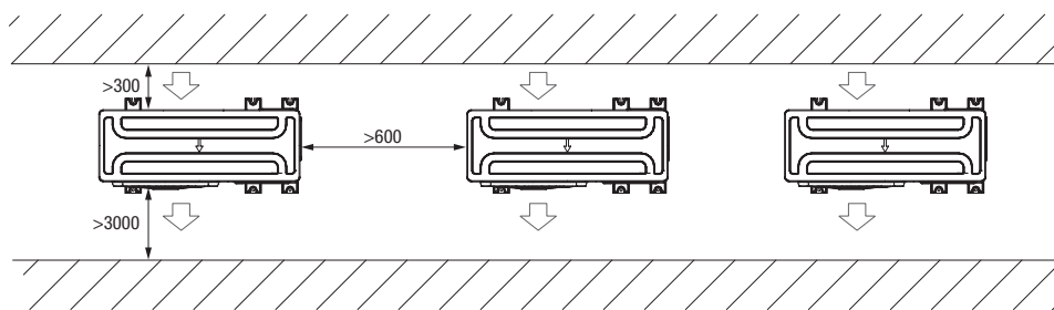
For parallel installation in a several row
