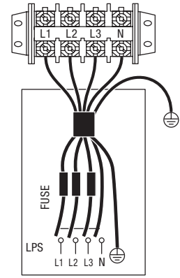
POWER SUPPLY 380VAC-3N
