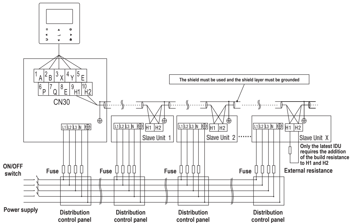
POWER SUPPLY 380VAC-3N
